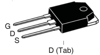
TO-247 (IXFH)
